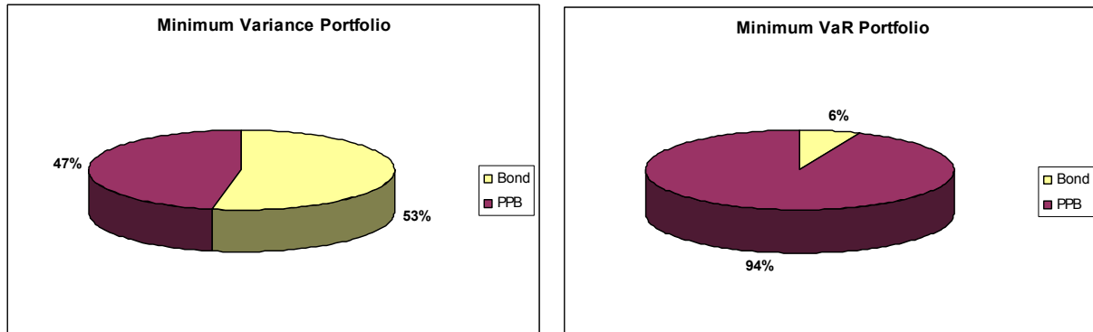
Figure 3: Composition of minimum risk portfolios
