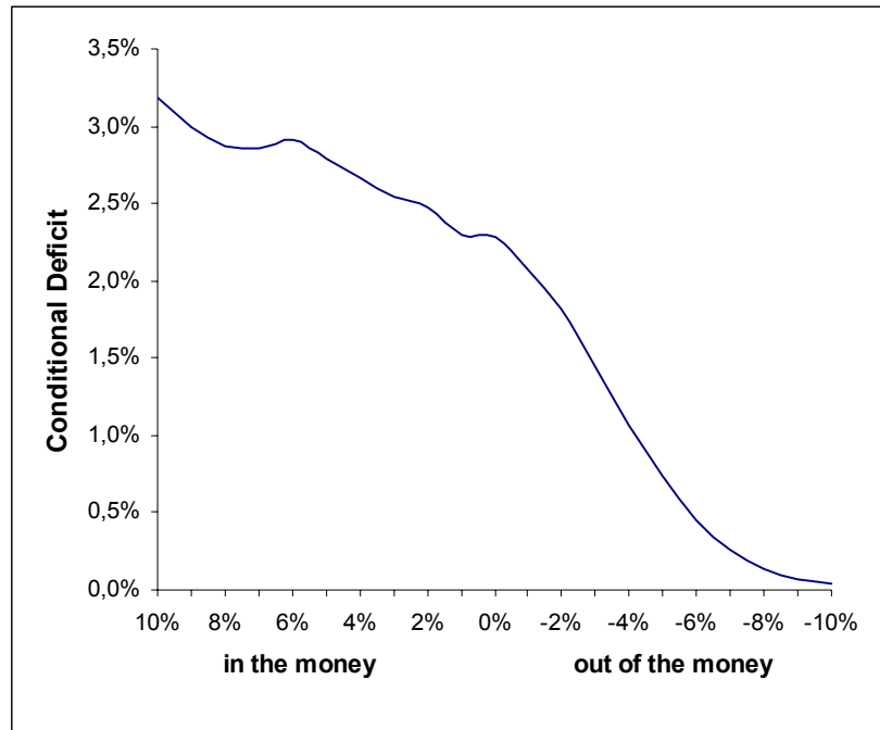
Figure 2: Conditional under-performance of the option strategy for different strike prices
