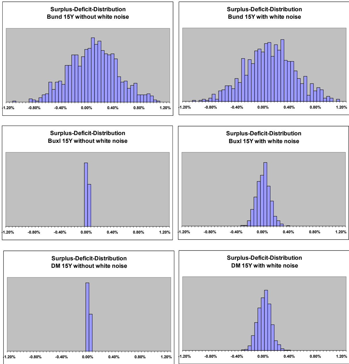
Figure 5: Surplus/Deficit between assets and liabilities after a three month period. 15 year duration for liabilities
