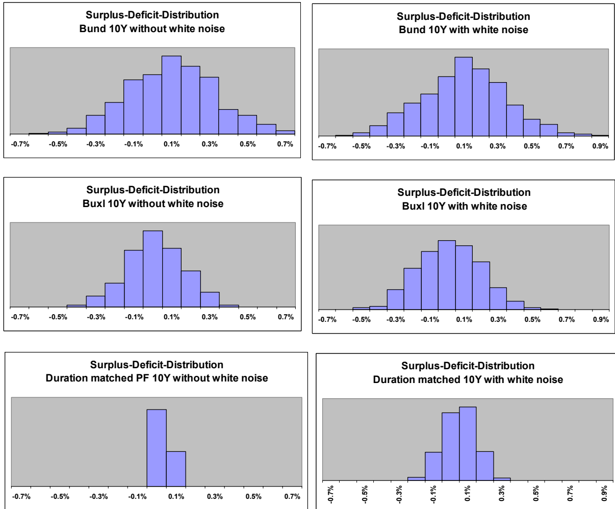
Figure 4: Surplus/Deficit between assets and liabilities after a three month period. 10 year duration for liabilities
